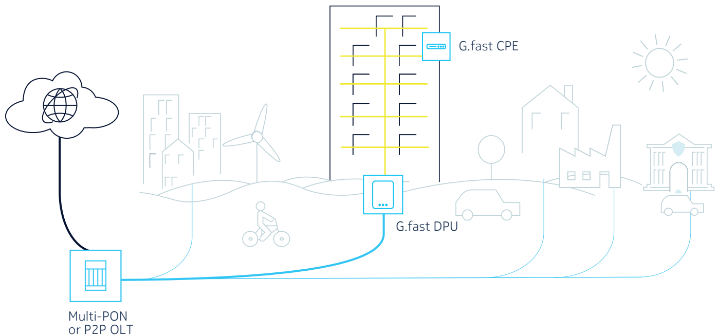
Figure 1. Typical G.fast deployment
