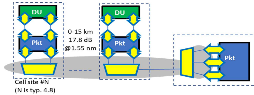
Figure 25: 15 km DRAN backhaul, DWDM passive wavelength multiplexed bus Blueprint. The link specified has a gray background. In cases where the cell site DU is collocated with the CU, backhaul is illustrated. If the CU is located at another location, HLS is illustrated.
