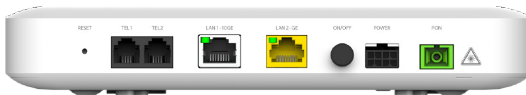
Figure 2: Nokia ONT XS-220X-A back view
