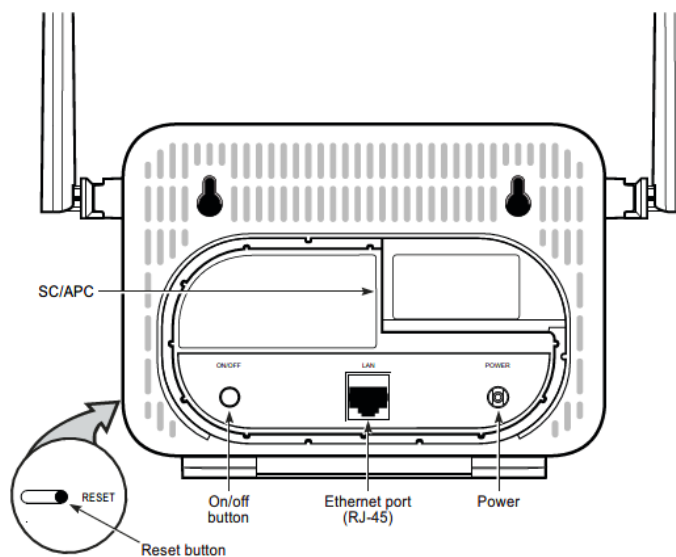
Figure 2: Nokia ONT G-0126G-A (back)
