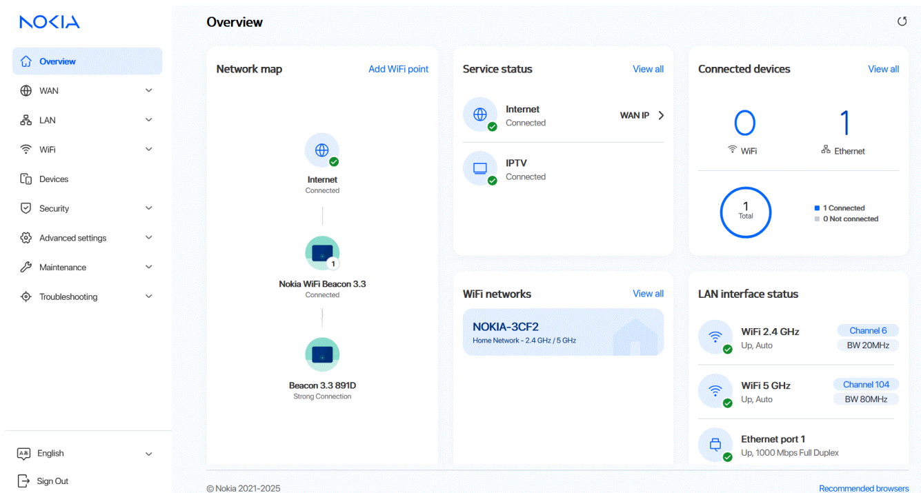
Figure 3 Nokia Wifi Beacon 3.3 WebGUI Overview screen
