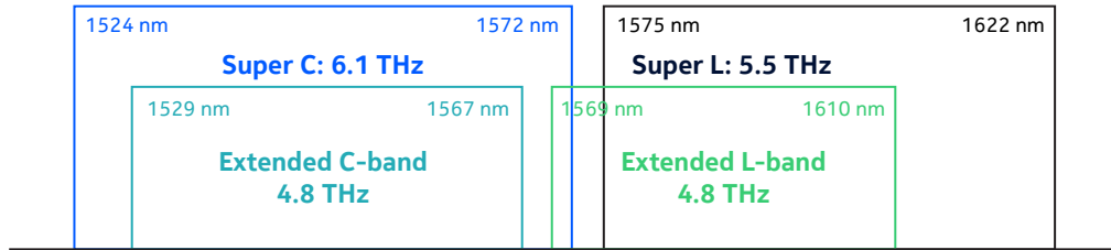
Figure 2 - Increased spectrum with L, Super C and Super L
