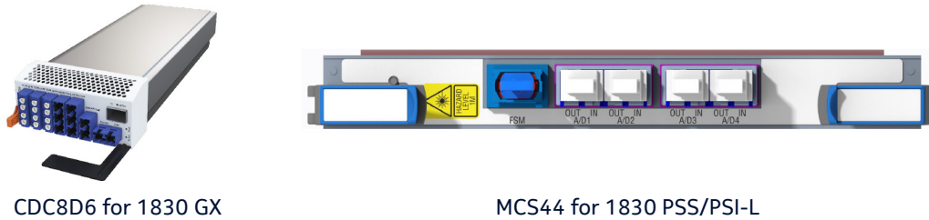
Figure 4 – Low-port-count CDC examples
