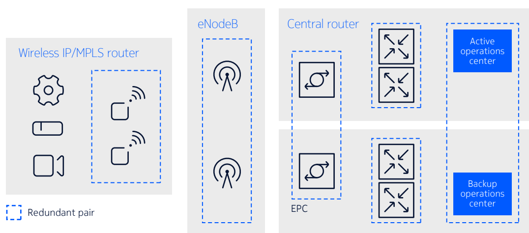
Figure 7. IP/MPLS enables a fully-protected, end-to-end communication path
