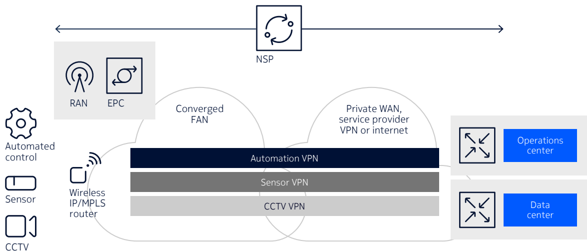
Figure 4. IP/MPLS VPN supports seamless end-to-end communication
