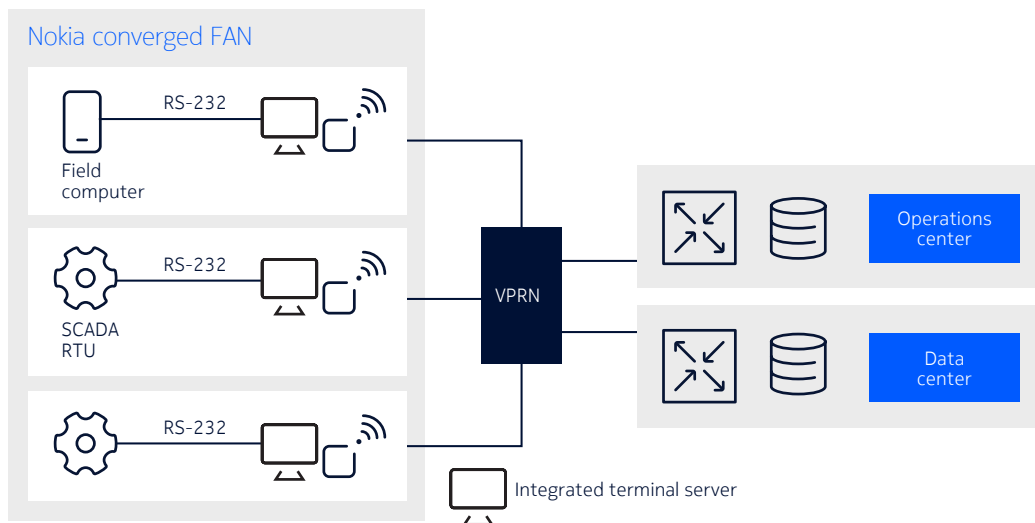
Figure 9. Raw socket technology for serial-to-IP seamless adaptation
