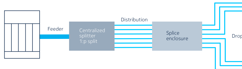
Figure 7. Centralized split PON architecture
