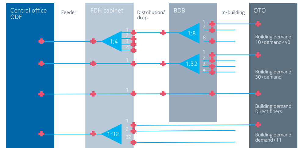
Figure 9. OSP architecture and splitting concept
