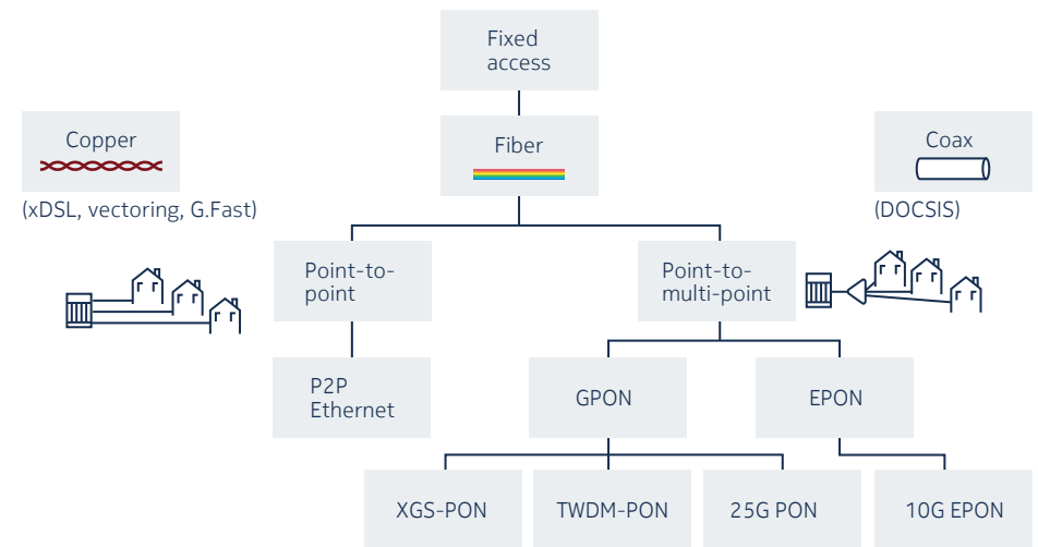
Figure 4. Overview of fiber access technologies
