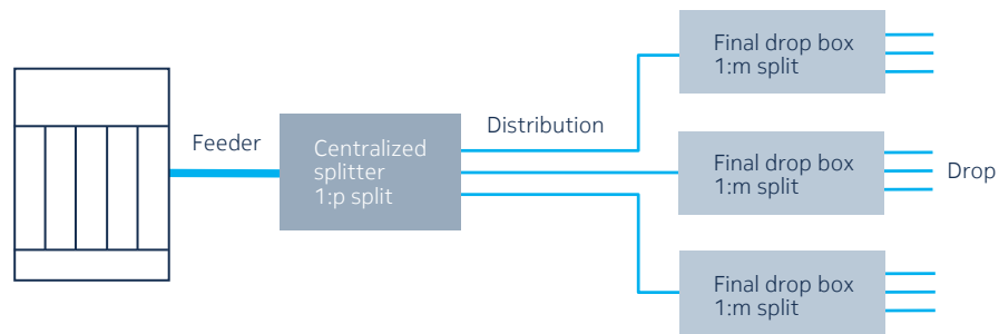
Figure 8. Cascaded or distributed split PON architecture
