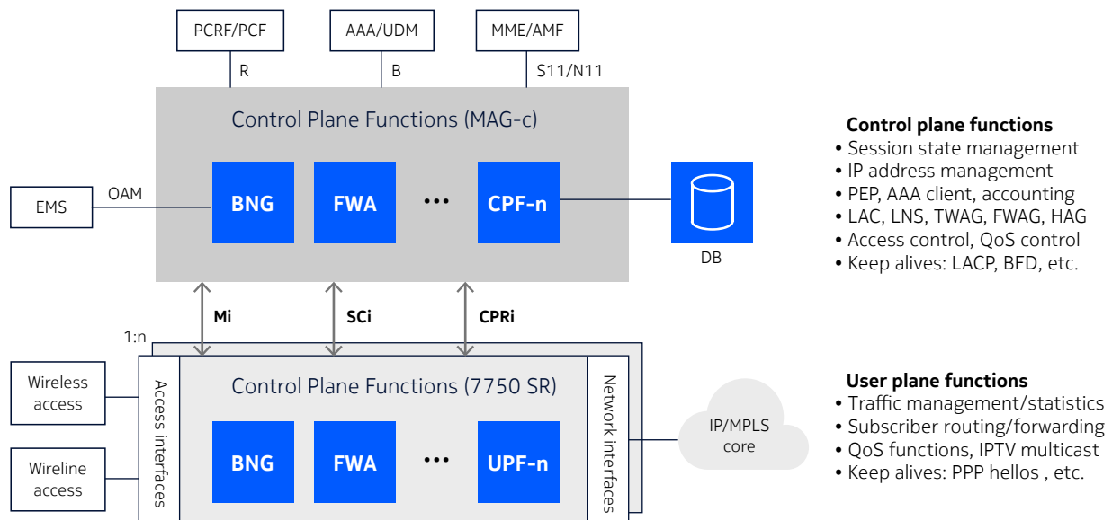
Figure 3. Disaggregated CUPS architecture (Broadband Forum TR-459)
