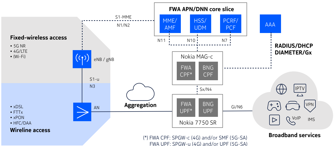
Figure 2. Multi-Access Gateway for wireline and converged operators
