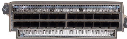
24-connector 200G SFP-DD MDA-se
