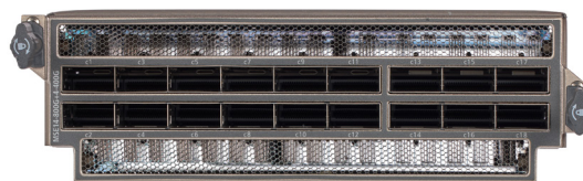
14-connector 800G QSFP-DD and 4-connector 400G QSFP112 MDA-se
